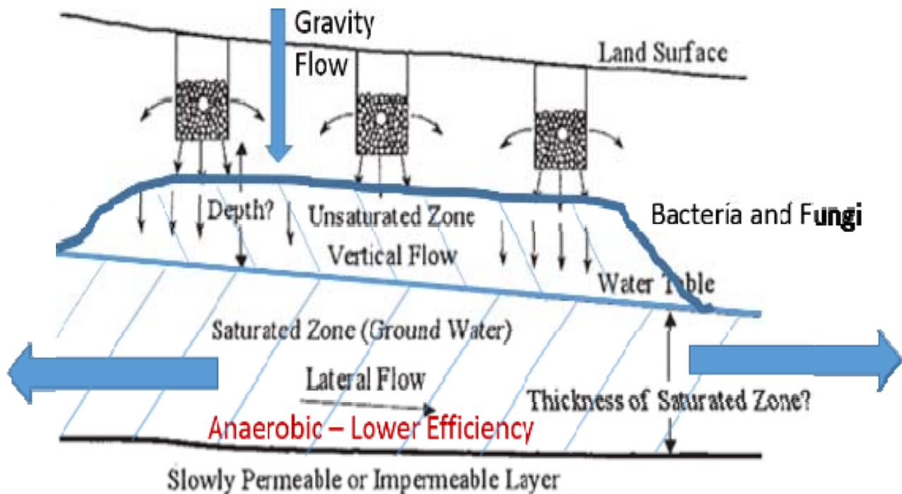
Figure 2. Addition of wastewater to the drain field artificially raises the groundwater table further restricting size of the unsaturated decontamination zone
